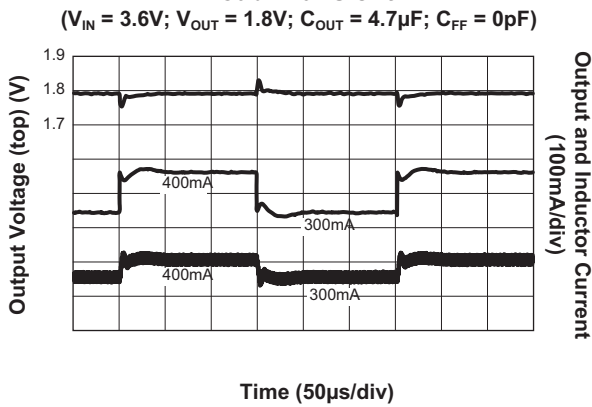
Load Transient
